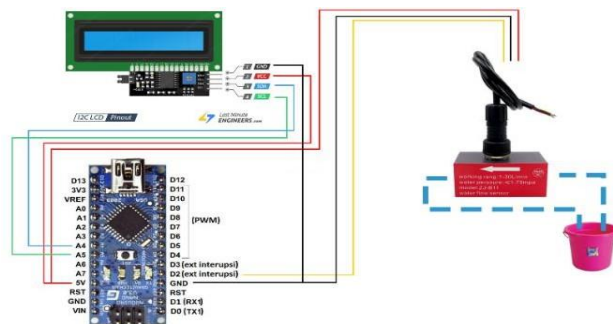
Figure 6. Schematic Diagram
