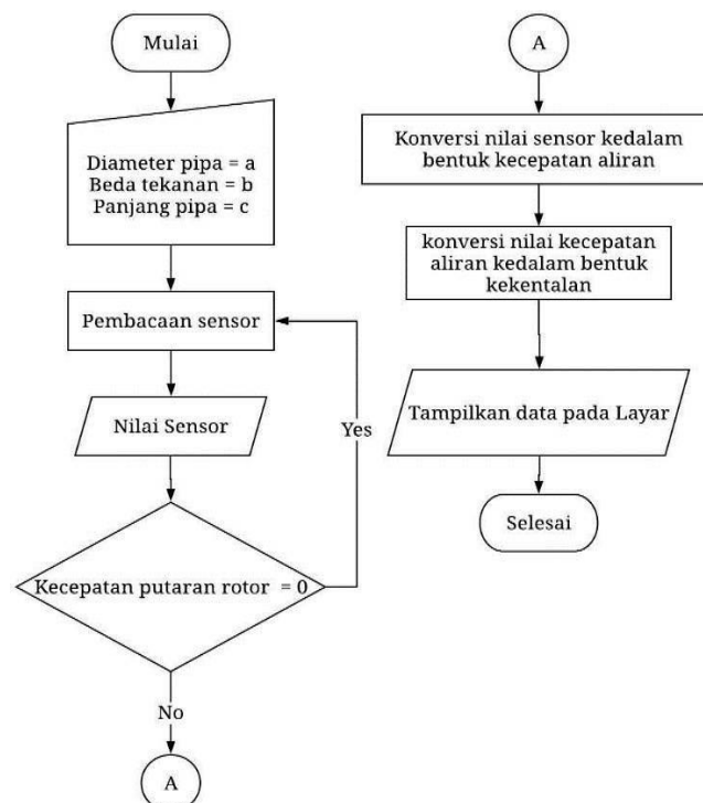
Figure 4. Program Flowchart
